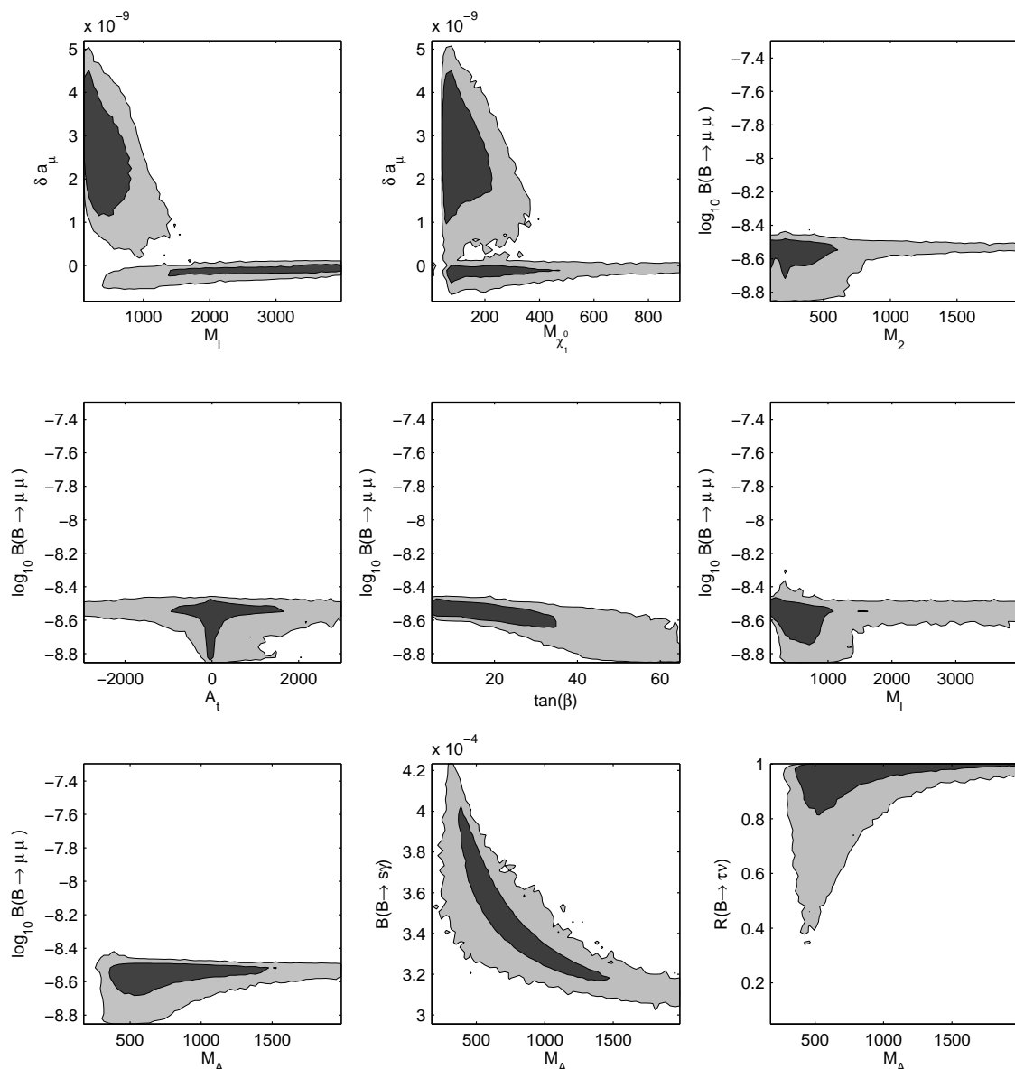
Figure 8. Same as figure 7 but with log prior. The 68% BC contour is in dark grey and the 95% BC contour in light grey.
