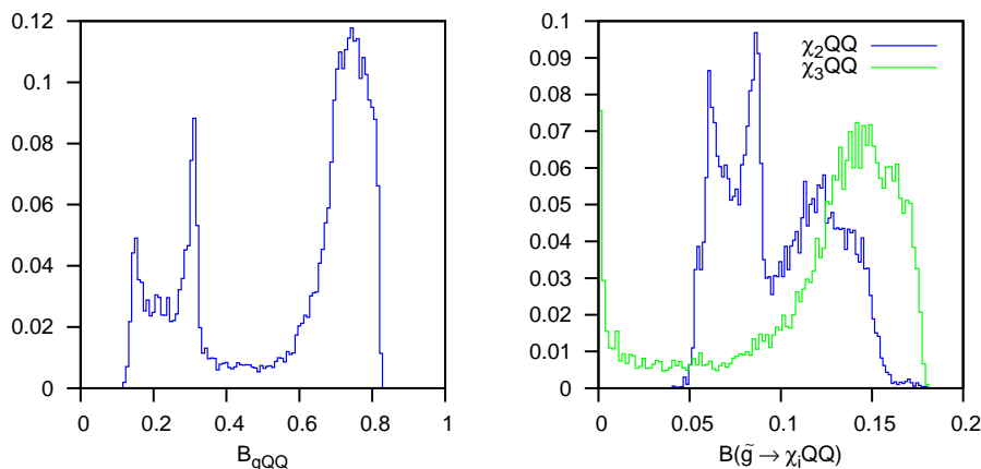
Figure 9. Distribution of the gluino branching fractions in third generation quarks a) B_{gQQ} b) Br(\tilde{g} \rightarrow \tilde{\chi}_i^0 QQ) . There is a scale factor of 10^6 on the y-axis.
