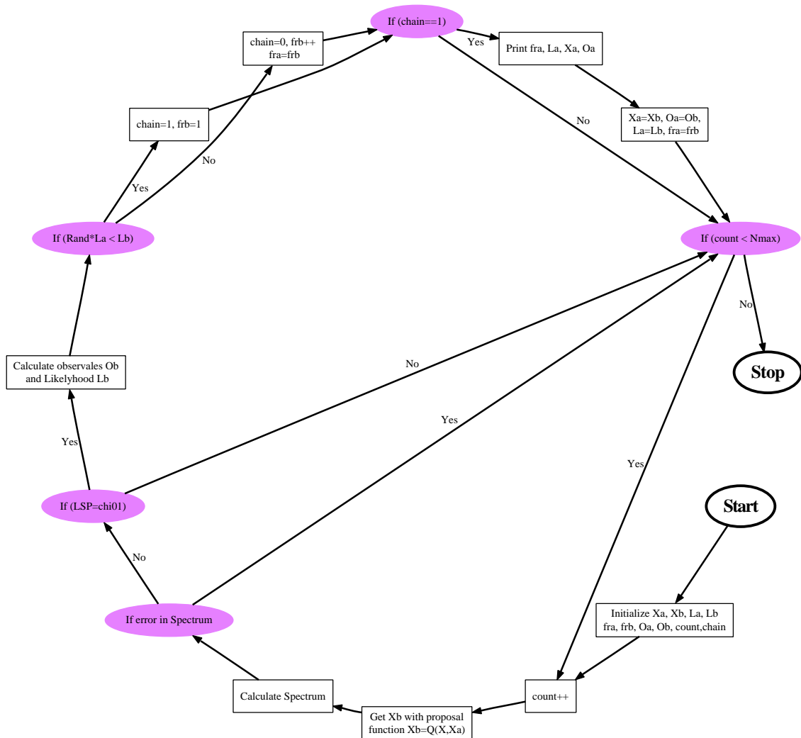
Figure 1. Details of the MCMC algorithm used in this paper. \mathbf{X}_a and \mathbf{X}_b are the points in the parameter space, O_a and O_b are the values of the observables at points \mathbf{X}_a and \mathbf{X}_b respectively, L_a and L_b are corresponding likelihoods and f_{ra} and f_{rb} are the frequencies at two points.
