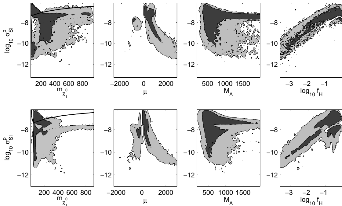
Figure 6. Predictions for elastic scattering cross sections as a function of m_{\tilde{\chi}_1^0} , \mu , M_A and f_H . Default values of micrOMEGAs2.2 for the quark content of the nucleon are taken. On the left panel the CDMS-II exclusion is shown by a solid line, while the dashed line shows the factor 10 improved limits. The top panel is with linear priors and the bottom panel with log priors.
