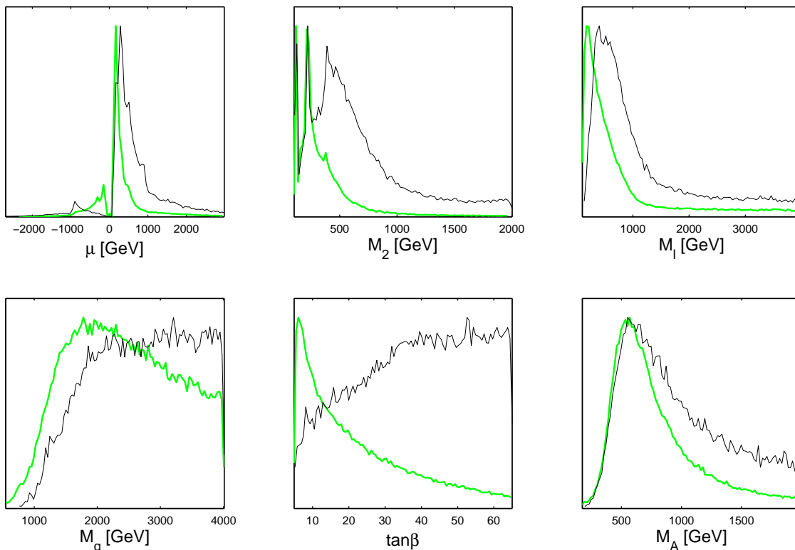
Figure 2. The posterior PDF of the model parameters is shown for linear priors (thin black line) and log priors (thick gray/green line).
