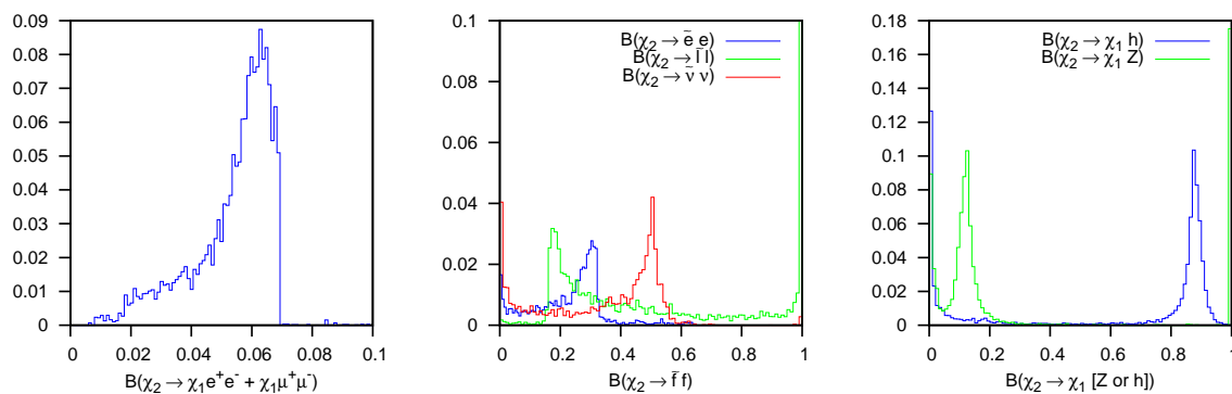
Figure 11. Distribution of \tilde{\chi}_2^0 branching fractions for the channels a) \tilde{\chi}_1^0 e^+ e^- (\mu^+ \mu^-) b) \tilde{l} \bar{l} c) \tilde{\chi}_1^0 Z, \tilde{\chi}_1^0 h . There is a scale factor of 10^6 on the y-axis.
