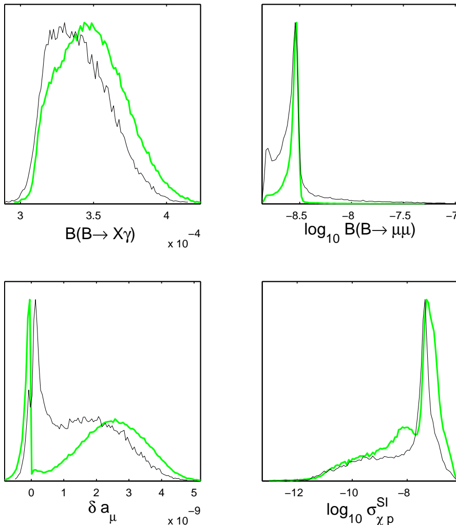
Figure 5. The posterior PDFs for B(b \rightarrow s\gamma) , B(B_s \rightarrow \mu^+\mu^-) , \delta a_\mu and \sigma_{\chi p}^{SI} . The scale on the y-axis is adjusted to have same maximum value for both linear priors (thin black line) and log priors (thick gray/green line).
