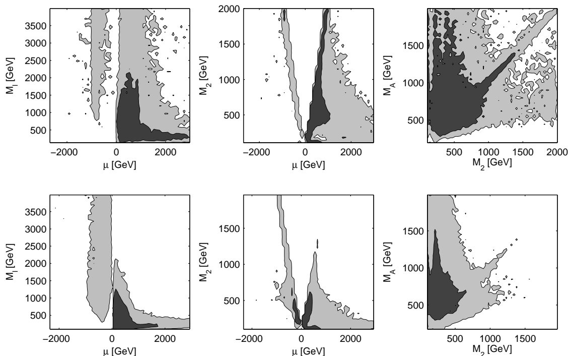
Figure 3. 2D contours for M_{\tilde{1}} - \mu (left panel) M_2 - \mu (middle panel) M_A - M_2 (right panel) showing the 68% BC (dark grey) and 95% BC (light grey) contours. The top panels are with linear priors and the bottom panels with log priors.
