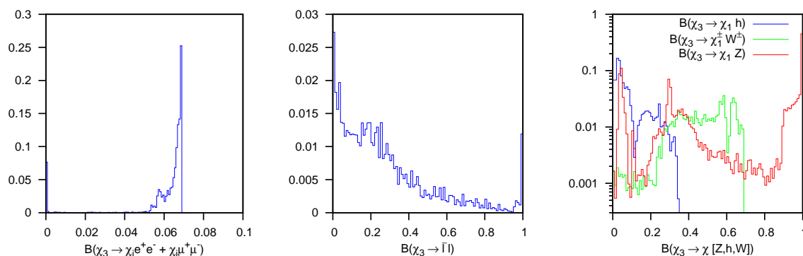
Figure 12. a) Distribution of \tilde{\chi}_3^0 branching fractions for the channels a) \tilde{\chi}_i^0 e^+ e^-, \mu^+ \mu^- b) \tilde{l} \bar{l} c) \tilde{\chi}_1^0 Z, \tilde{\chi}_1^0 h, \tilde{\chi}_1^0 W . There is a scale factor of 10^6 on the y-axis.
