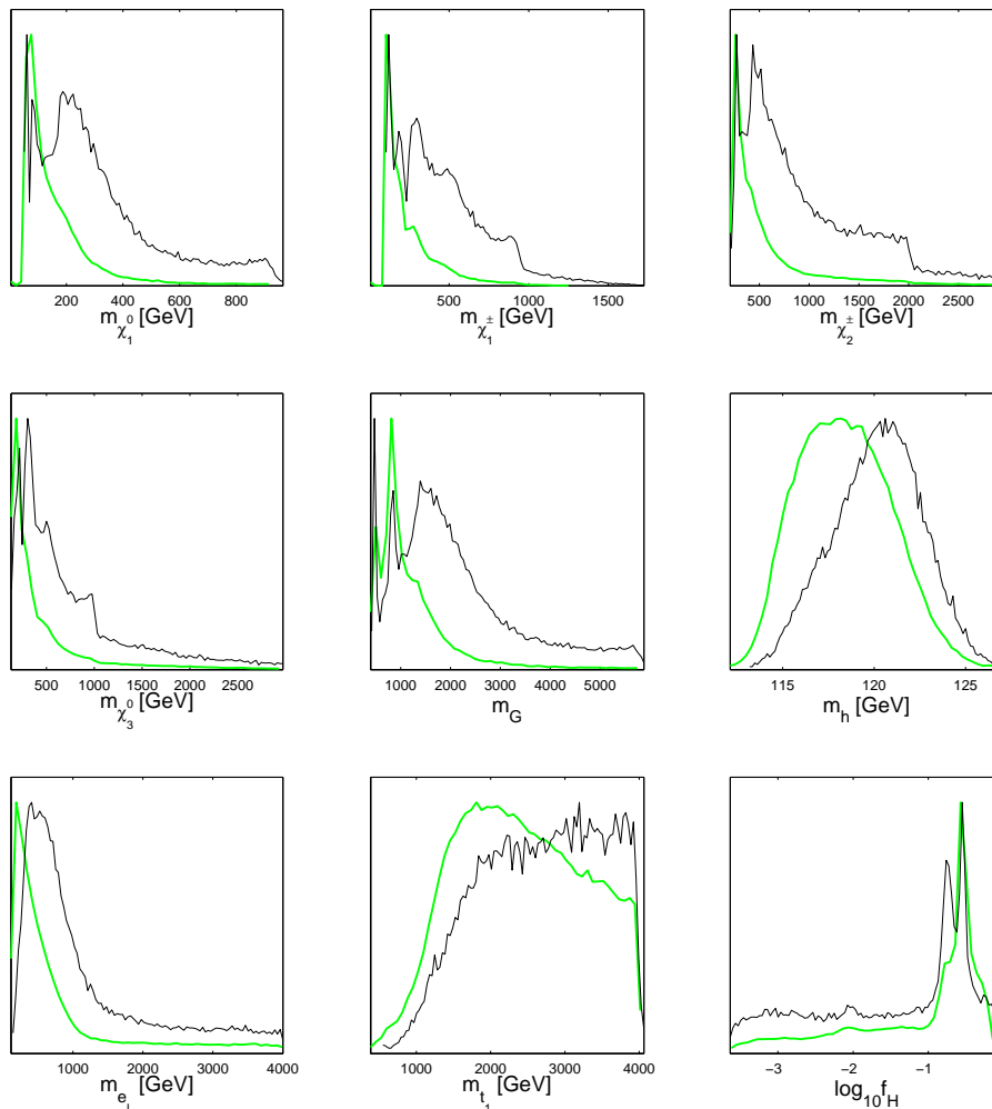
Figure 4. The posterior PDFs for sparticle masses: m_{\tilde{\chi}_1^0}, m_{\tilde{\chi}_1^\pm}, m_{\tilde{\chi}_3^0}, m_{\tilde{\chi}_2^\pm}, m_{\tilde{g}}, m_h, m_{\tilde{e}_L}, m_{\tilde{t}_1} and for the higgsino fraction, f_H . The scale on the y-axis is adjusted to have same maximum value for both linear priors (thin black line) and log priors (thick gray/green line).
